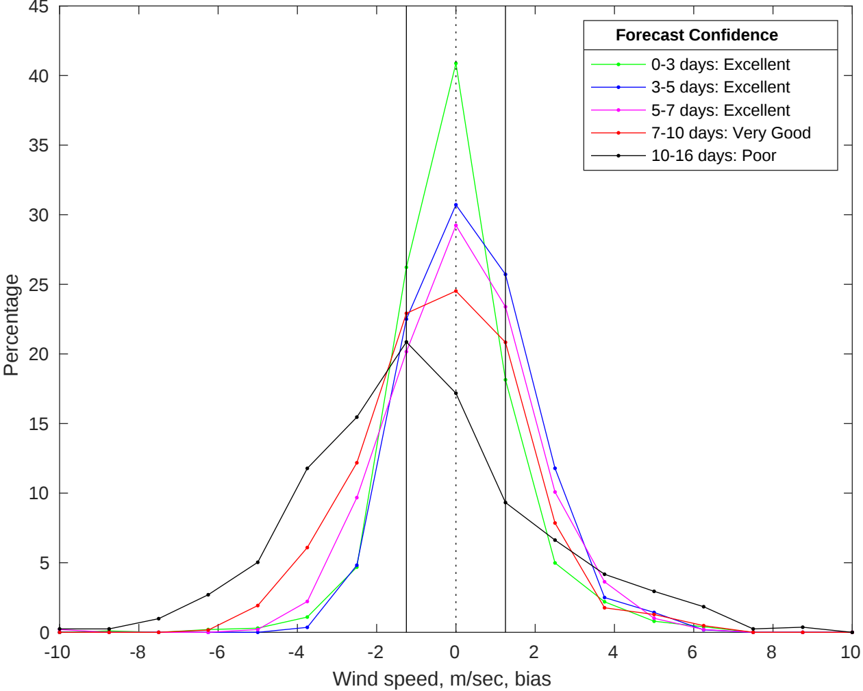
NDBC 42020 vs GFS Winds Bias Histogram: 18-Jun-2025
