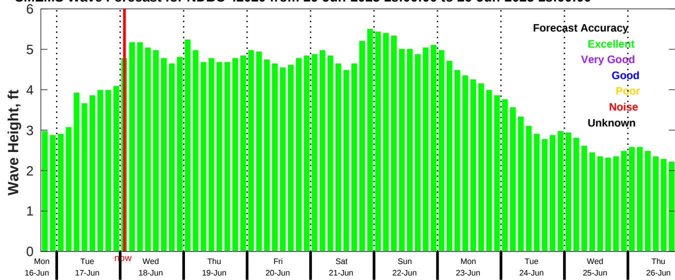
CMEMS Wave Forecast for NDBC 42020 from 16-Jun-2025 18:00:00 to 26-Jun-2025 18:00:00
