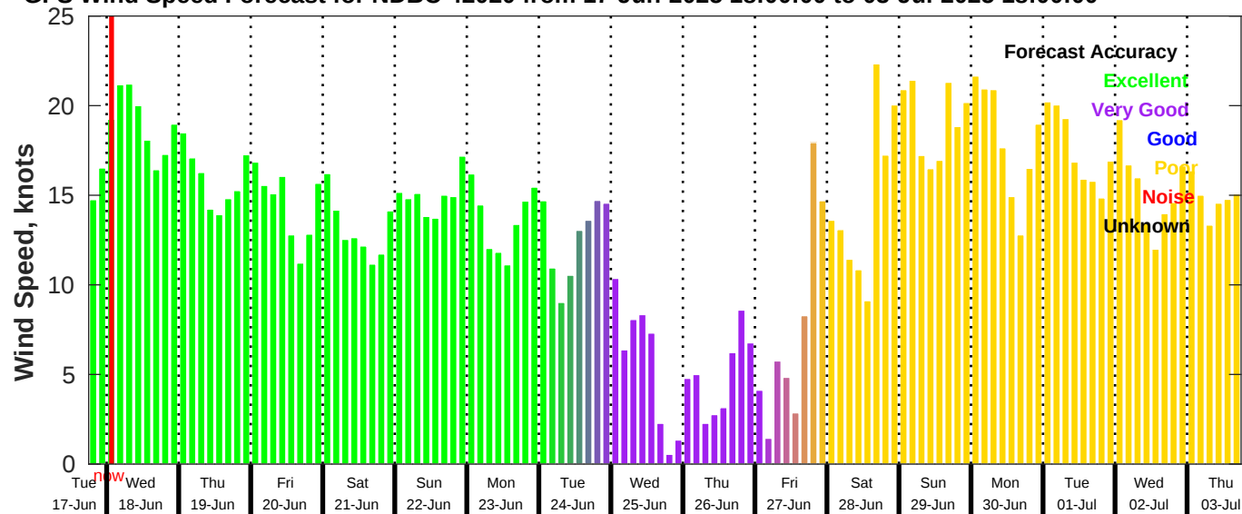
GFS Wind Speed Forecast for NDBC 42020 from 17-Jun-2025 18:00:00 to 03-Jul-2025 18:00:00
