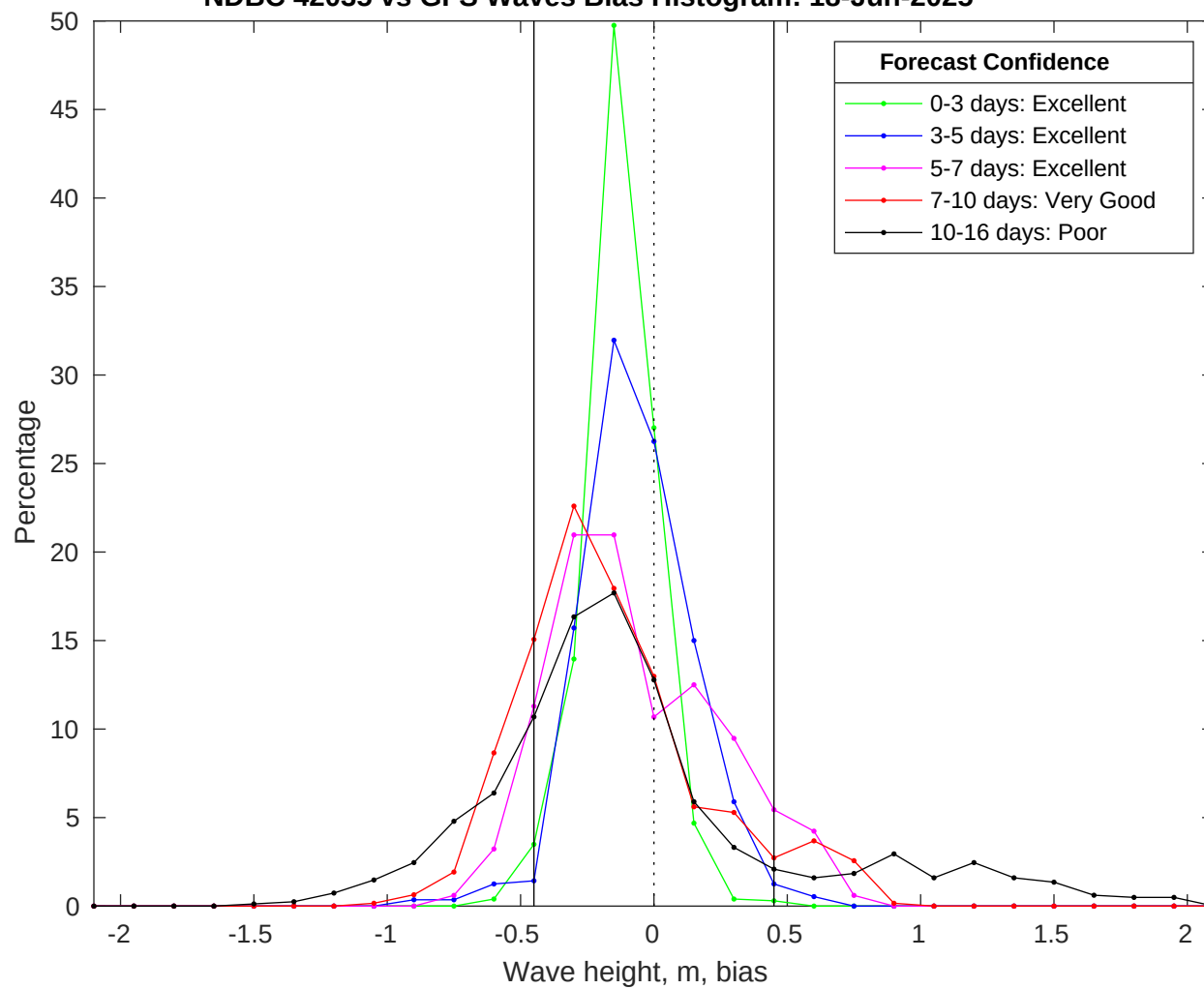
NDBC 42035 vs GFS Waves Bias Histogram: 18-Jun-2025
