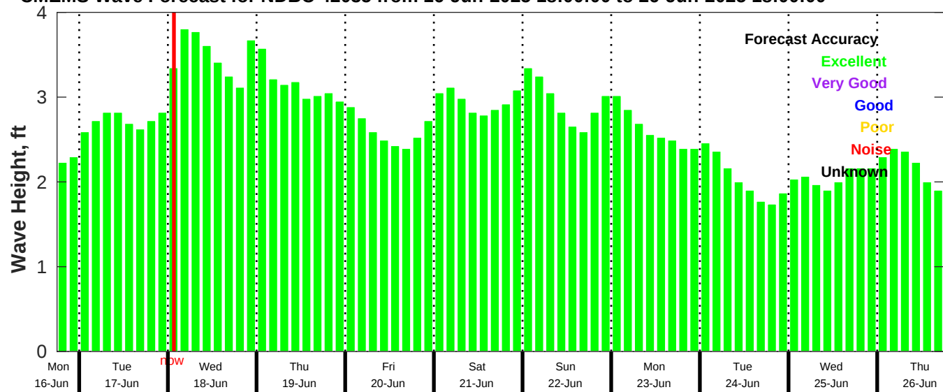
CMEMS Wave Forecast for NDBC 42035 from 16-Jun-2025 18:00:00 to 26-Jun-2025 18:00:00
