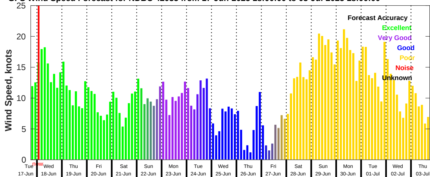
GFS Wind Speed Forecast for NDBC 42035 from 17-Jun-2025 18:00:00 to 03-Jul-2025 18:00:00
