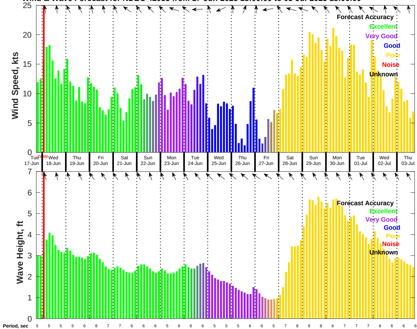
Wind & Wave Forecast for NDBC 42035 from 17-Jun-2025 18:00:00 to 03-Jul-2025 18:00:00
