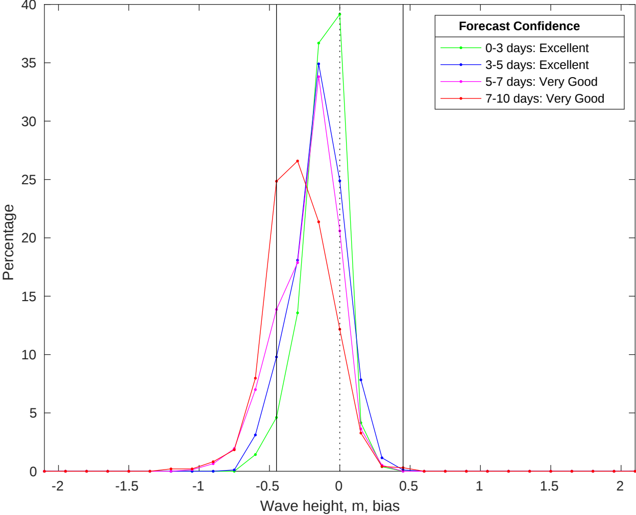
NDBC 42036 vs CMEMS Waves Bias Histogram: 18-Jun-2025
