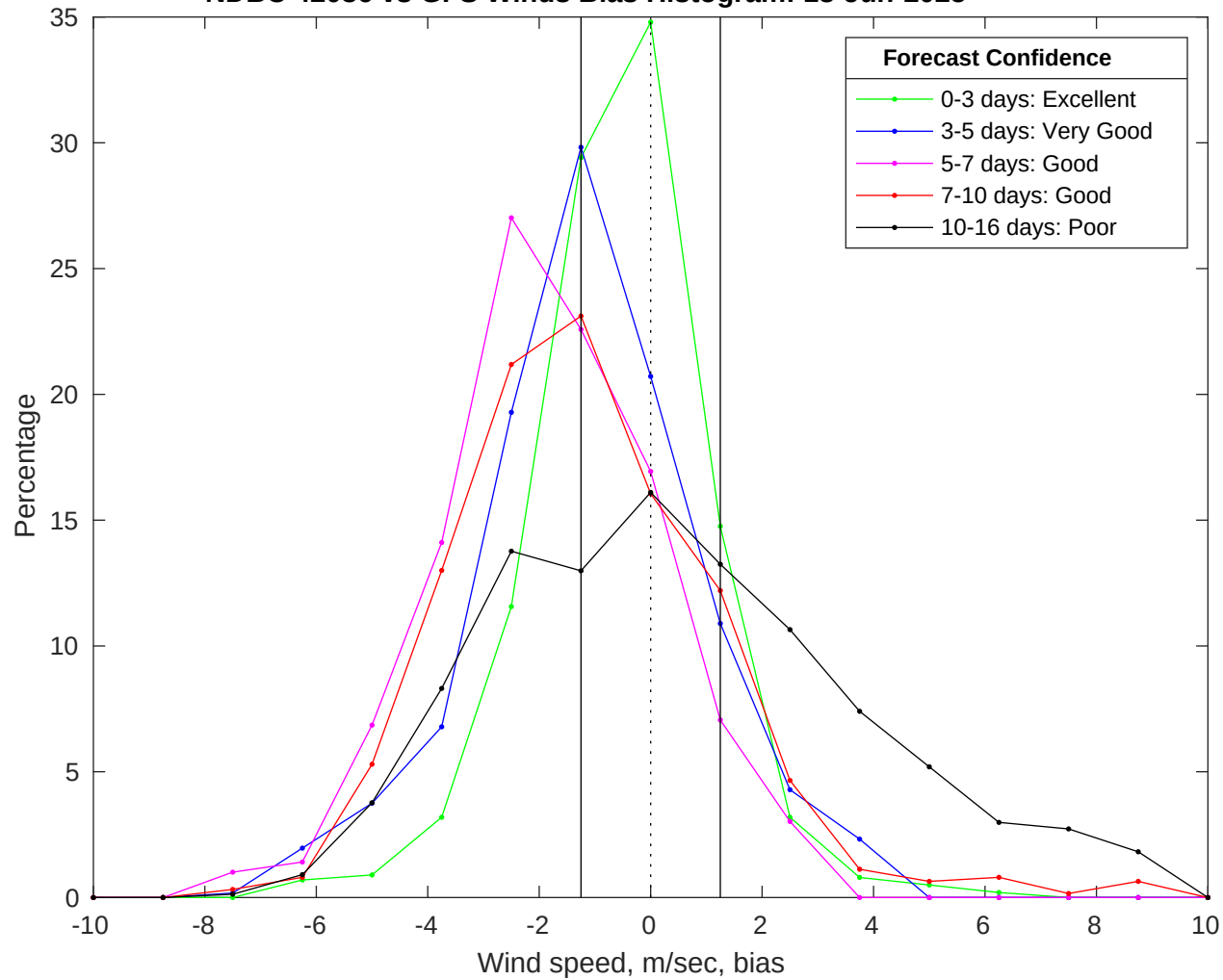
NDBC 42036 vs GFS Winds Bias Histogram: 18-Jun-2025
