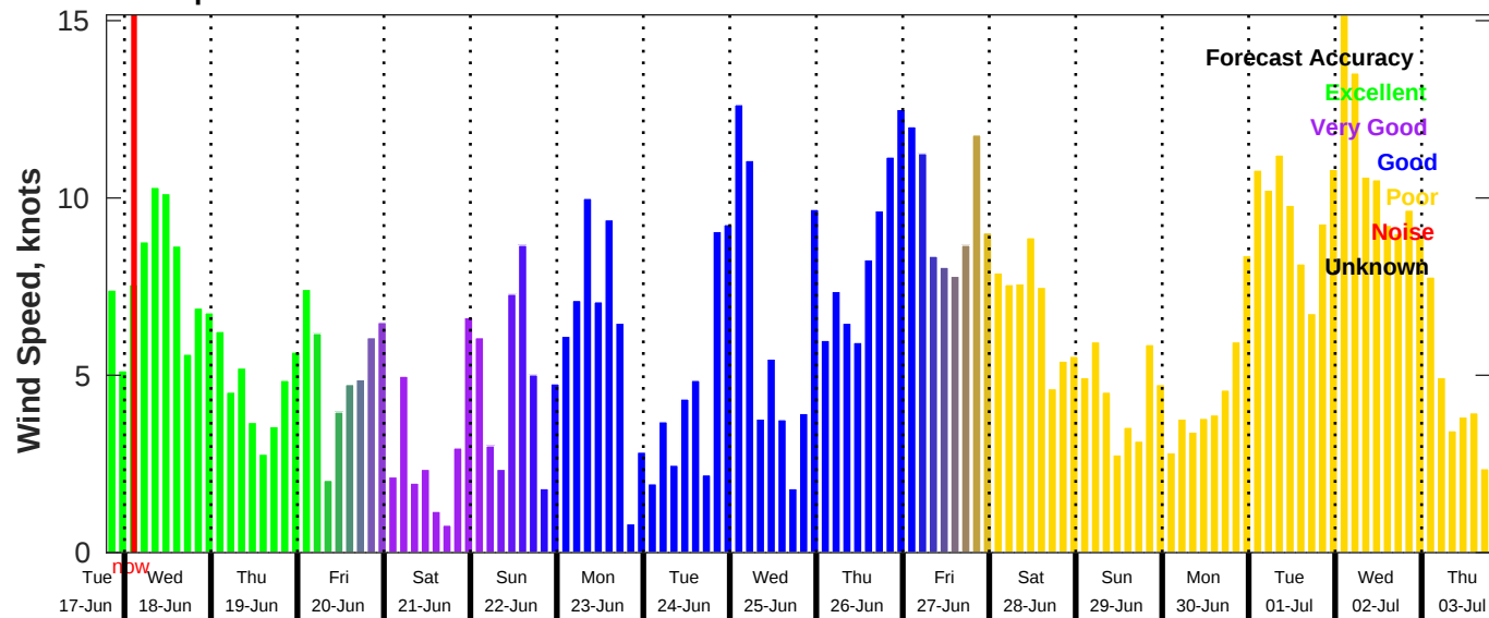
GFS Wind Speed Forecast for NDBC 42036 from 17-Jun-2025 19:00:00 to 03-Jul-2025 19:00:00
