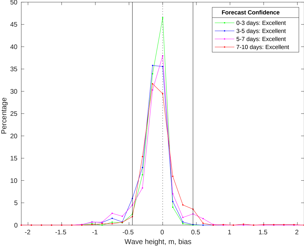
NDBC 42040 vs CMEMS Waves Bias Histogram: 18-Jun-2025
