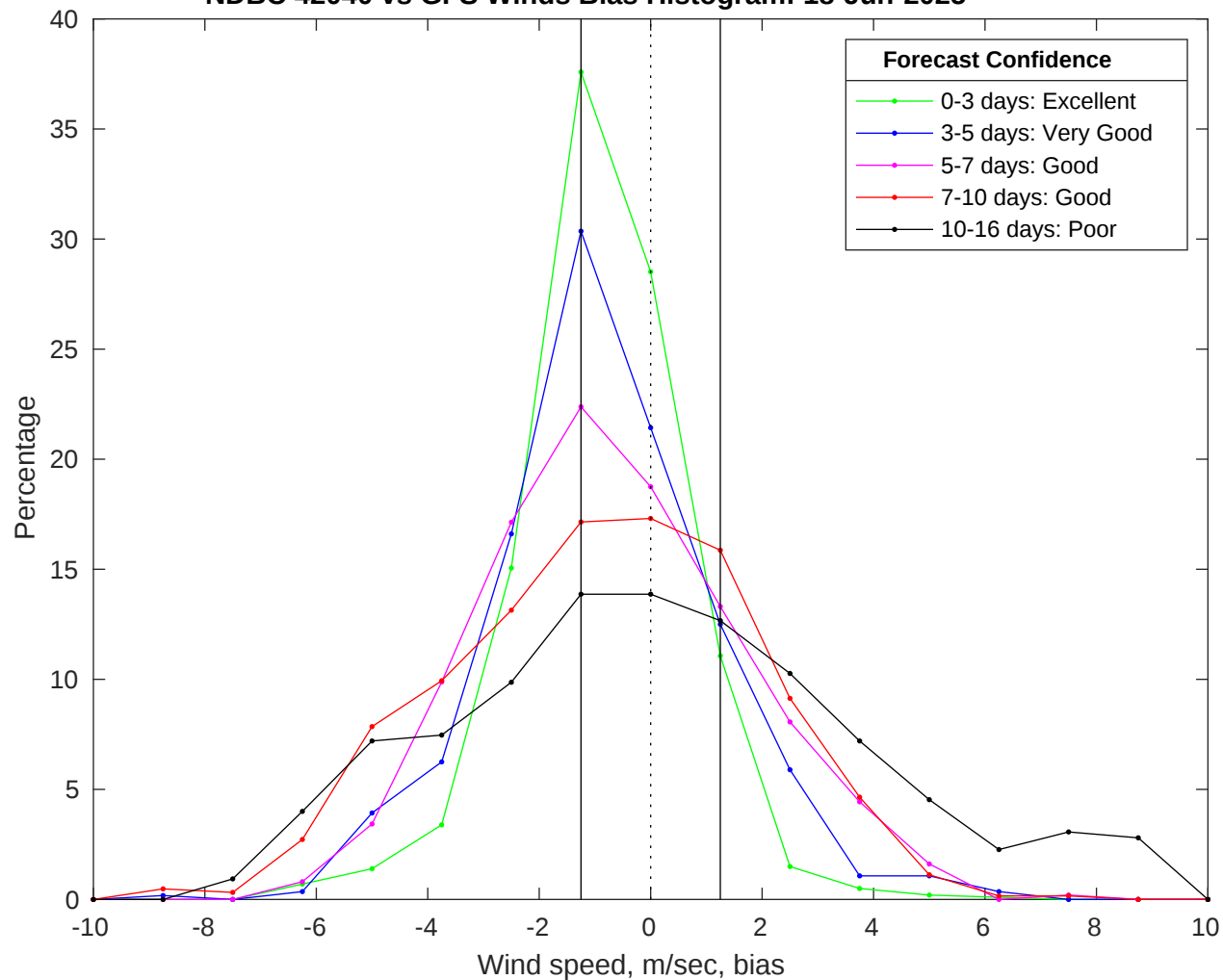
NDBC 42040 vs GFS Winds Bias Histogram: 18-Jun-2025
