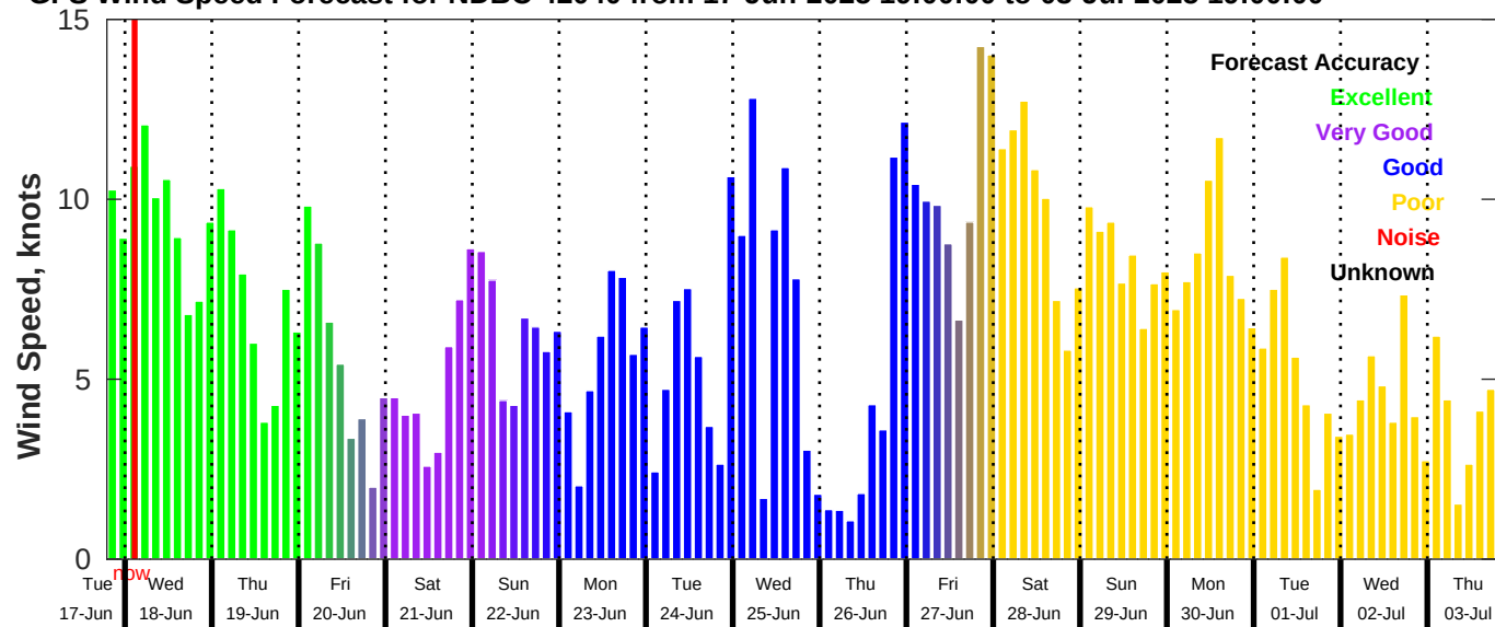
GFS Wind Speed Forecast for NDBC 42040 from 17-Jun-2025 19:00:00 to 03-Jul-2025 19:00:00
