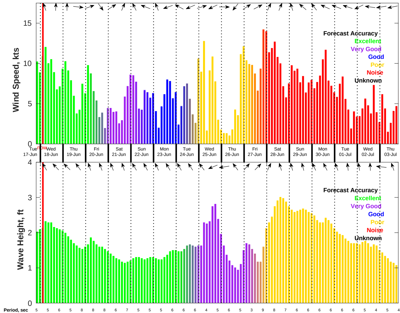
Wind & Wave Forecast for NDBC 42040 from 17-Jun-2025 19:00:00 to 03-Jul-2025 19:00:00
