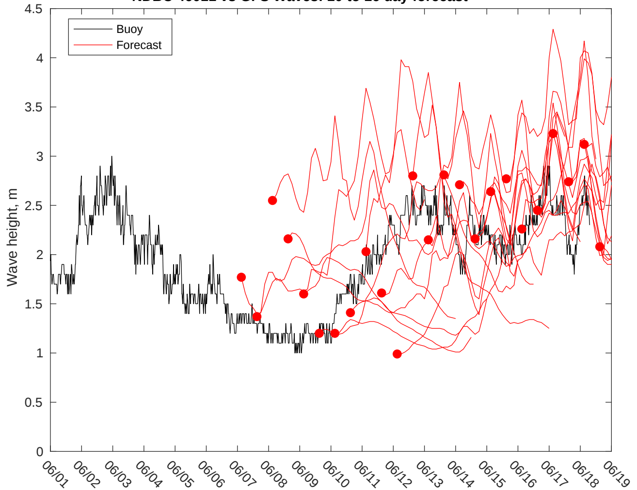
NDBC 46011 vs GFS Waves: 10 to 16 day forecast
