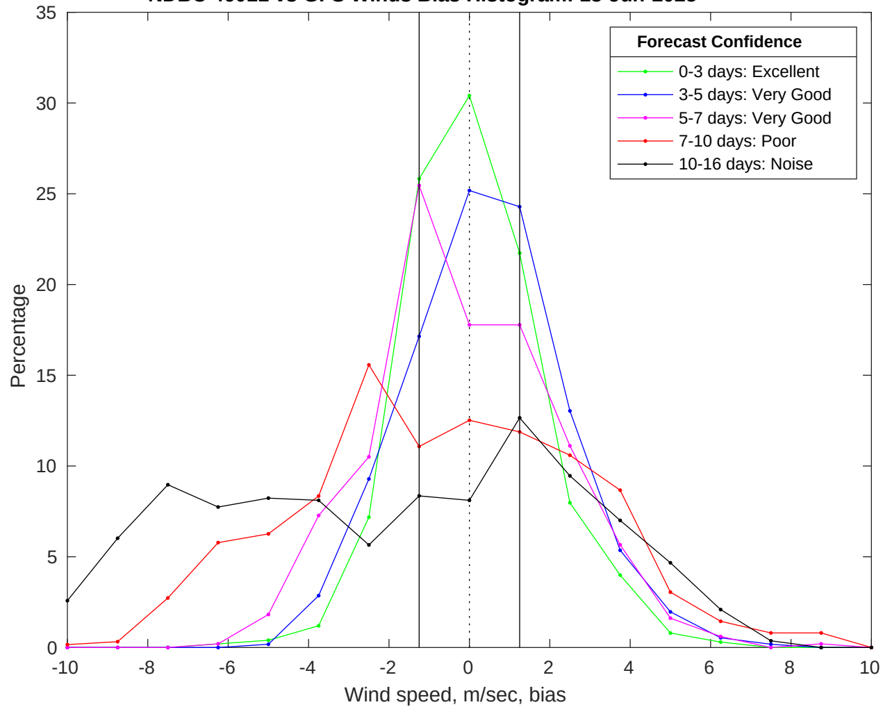
NDBC 46011 vs GFS Winds Bias Histogram: 18-Jun-2025
