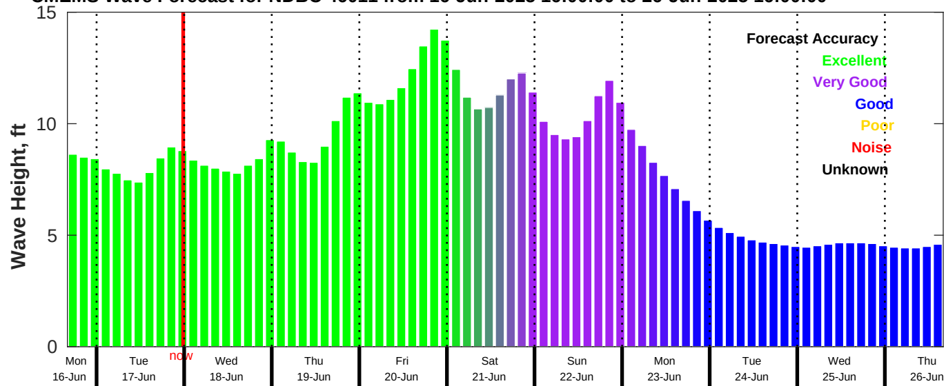
CMEMS Wave Forecast for NDBC 46011 from 16-Jun-2025 16:00:00 to 26-Jun-2025 16:00:00
