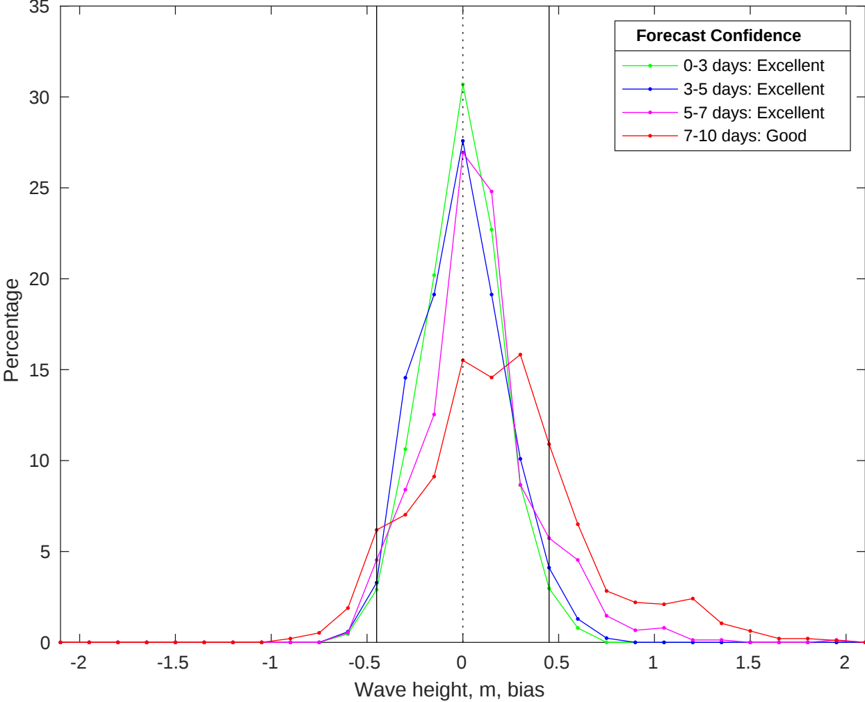
NDBC 46028 vs CMEMS Waves Bias Histogram: 18-Jun-2025
