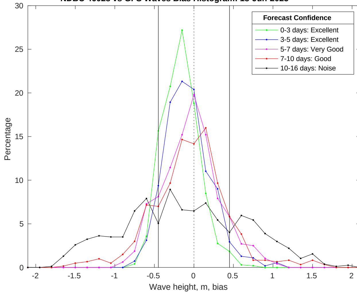
NDBC 46028 vs GFS Waves Bias Histogram: 18-Jun-2025
