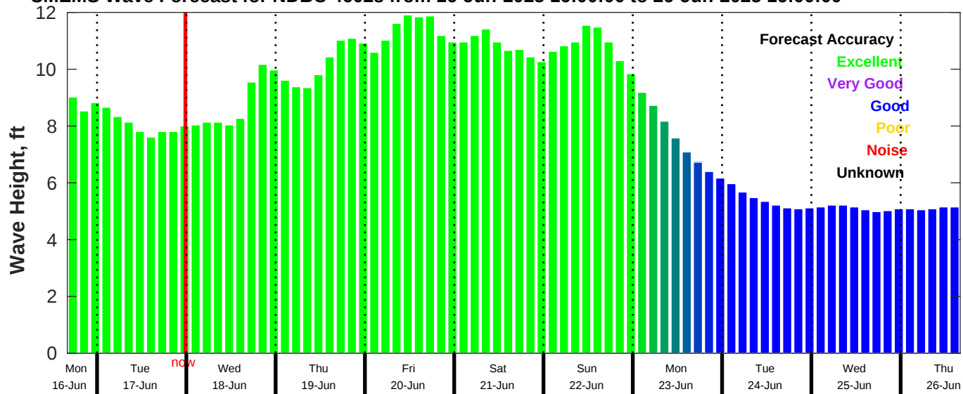
CMEMS Wave Forecast for NDBC 46028 from 16-Jun-2025 16:00:00 to 26-Jun-2025 16:00:00
