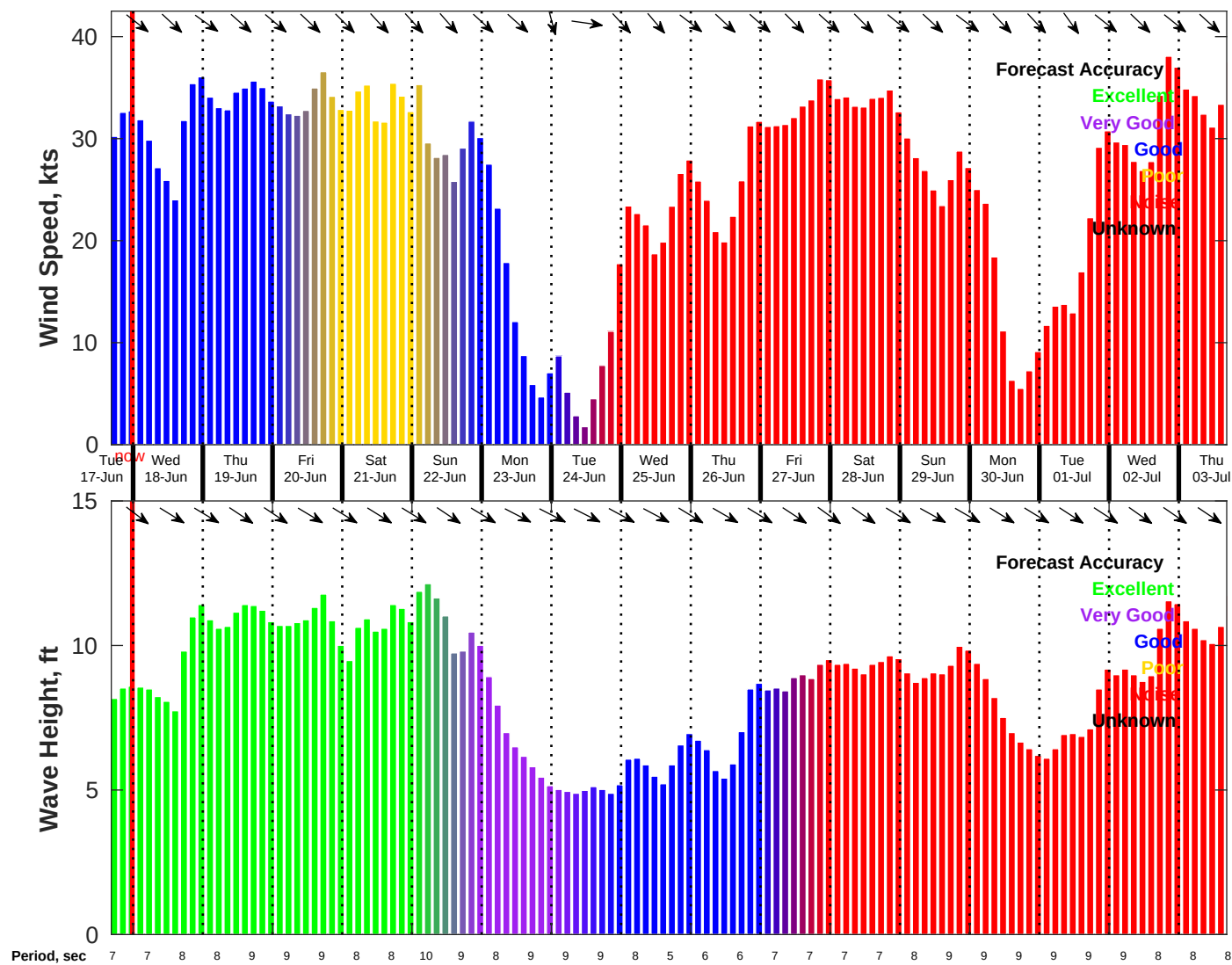
Wind & Wave Forecast for NDBC 46028 from 17-Jun-2025 16:00:00 to 03-Jul-2025 16:00:00
