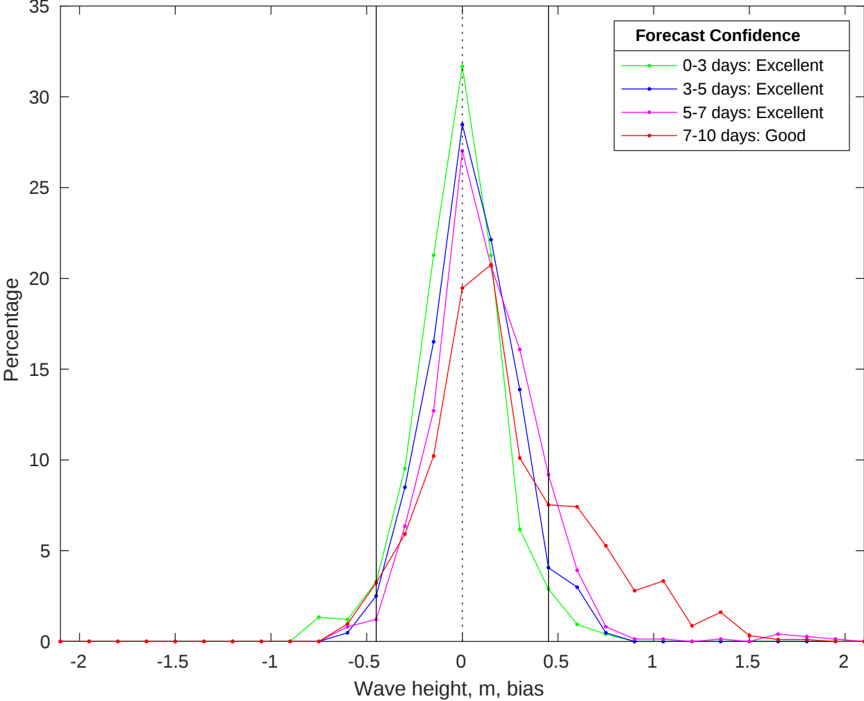
NDBC 46054 vs CMEMS Waves Bias Histogram: 18-Jun-2025
