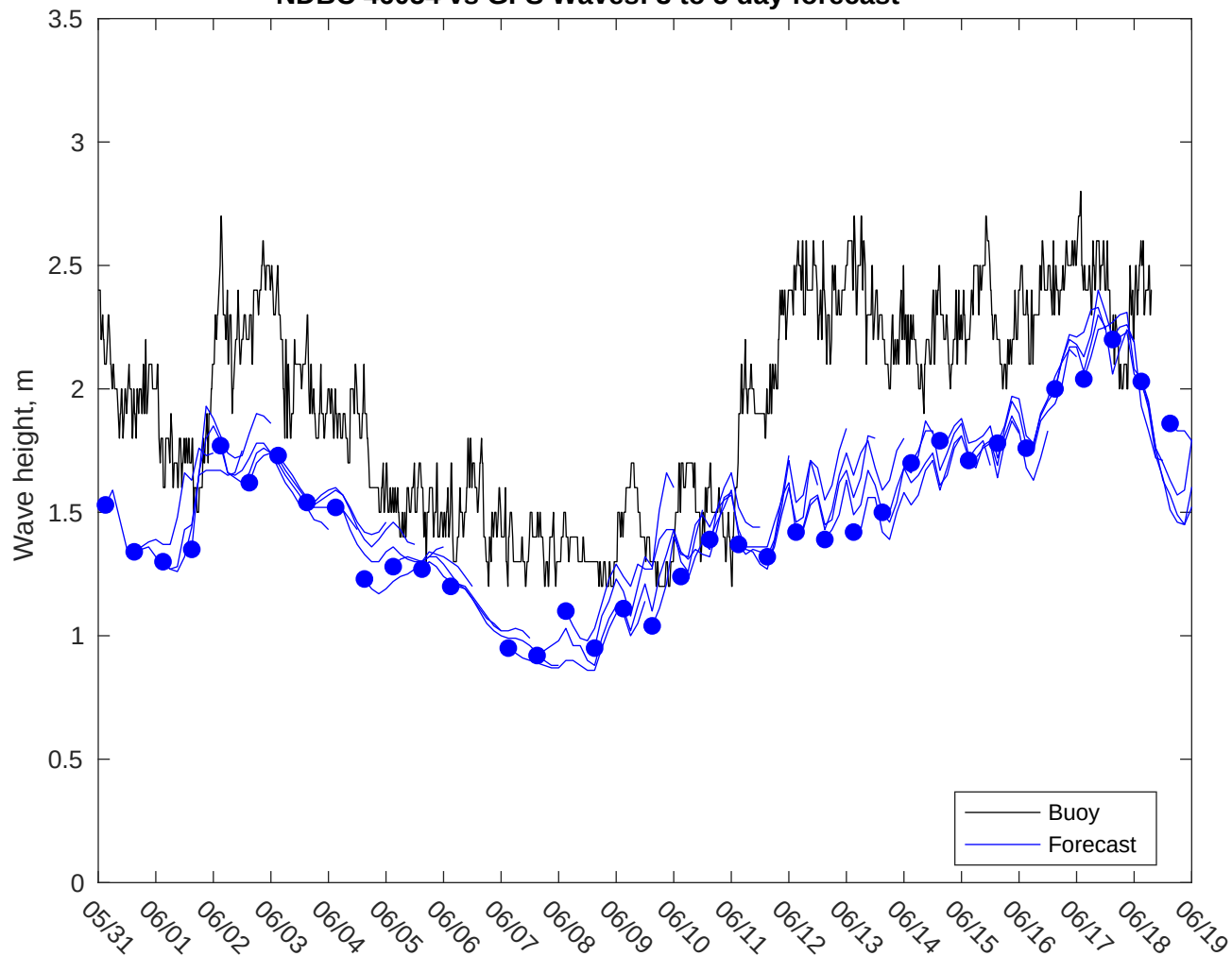
NDBC 46054 vs GFS Waves: 3 to 5 day forecast
