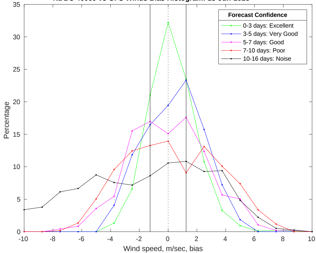
NDBC 46069 vs GFS Winds Bias Histogram: 18-Jun-2025
