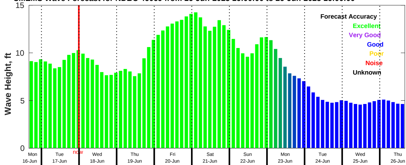
CMEMS Wave Forecast for NDBC 46069 from 16-Jun-2025 16:00:00 to 26-Jun-2025 16:00:00
