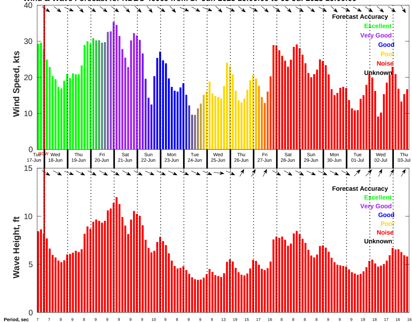
Wind & Wave Forecast for NDBC 46069 from 17-Jun-2025 16:00:00 to 03-Jul-2025 16:00:00
