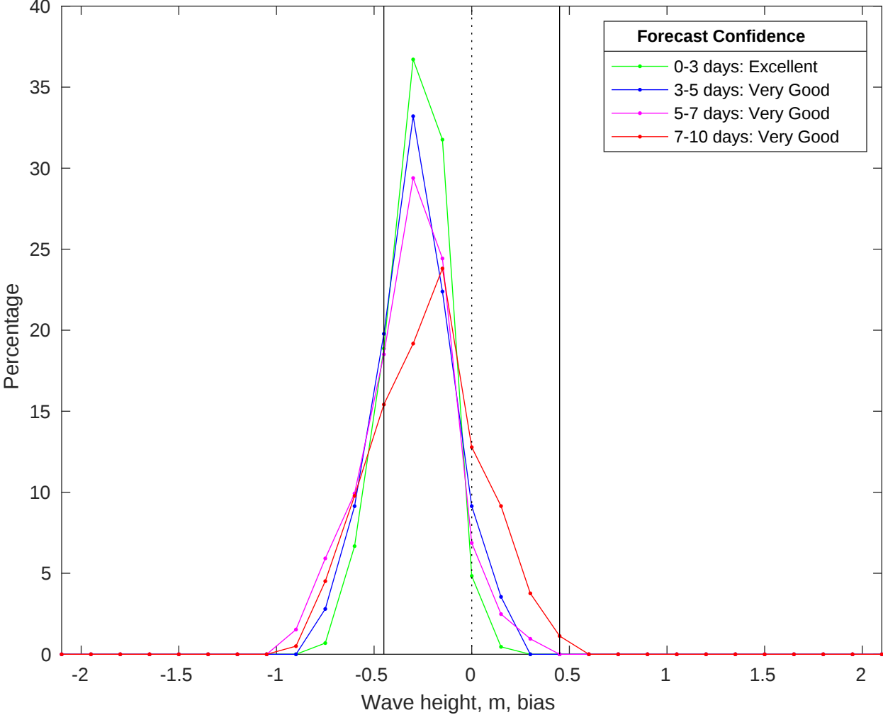
NDBC 51209 vs CMEMS Waves Bias Histogram: 18-Jun-2025
