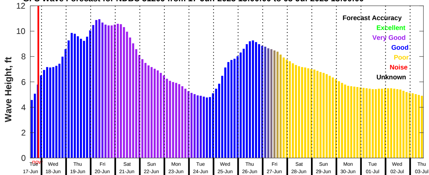
GFS Wave Forecast for NDBC 51209 from 17-Jun-2025 13:00:00 to 03-Jul-2025 13:00:00
