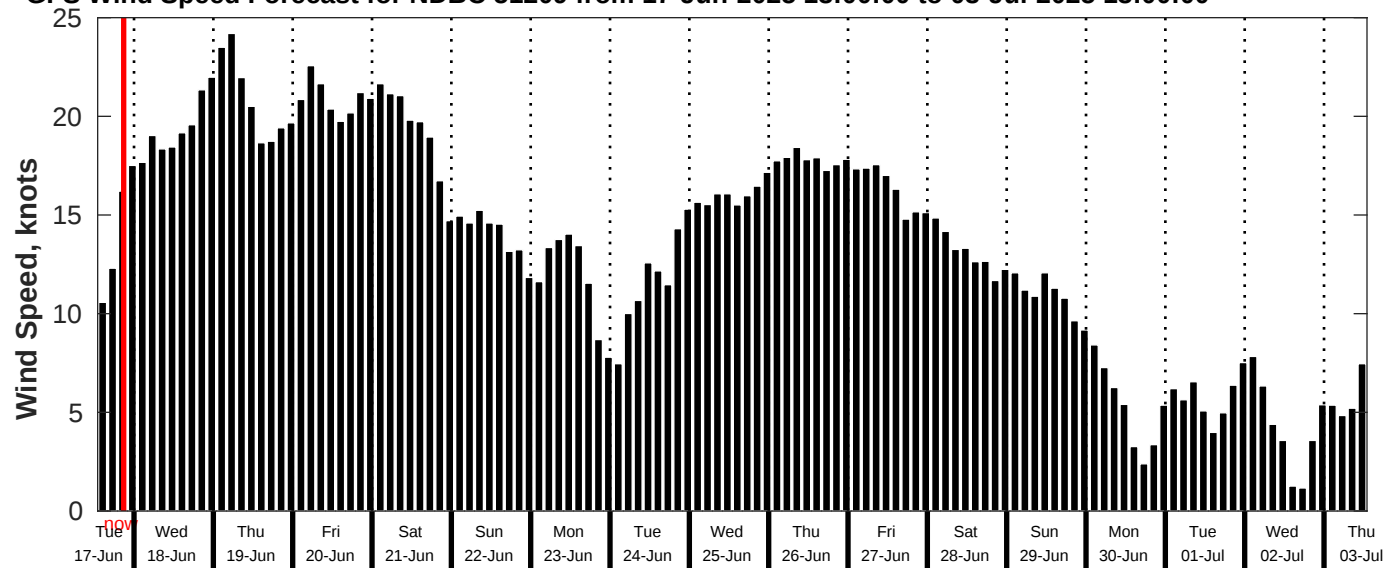
GFS Wind Speed Forecast for NDBC 51209 from 17-Jun-2025 13:00:00 to 03-Jul-2025 13:00:00
