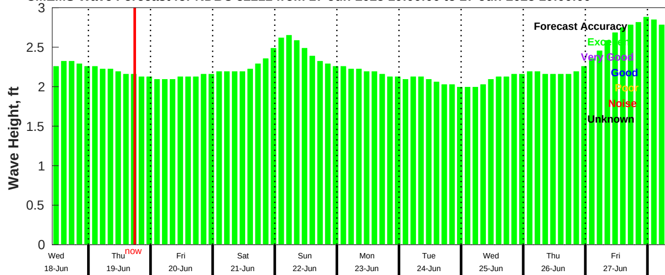
CMEMS Wave Forecast for NDBC 52211 from 17-Jun-2025 10:00:00 to 27-Jun-2025 10:00:00
