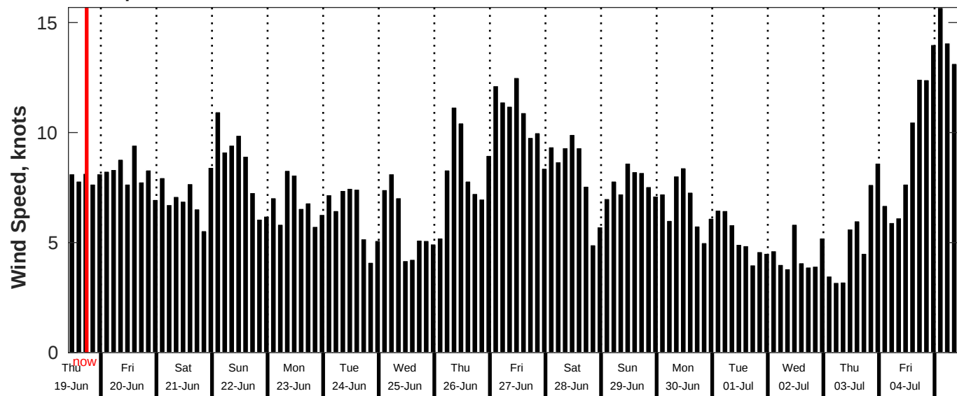
GFS Wind Speed Forecast for NDBC 52211 from 18-Jun-2025 10:00:00 to 04-Jul-2025 10:00:00
