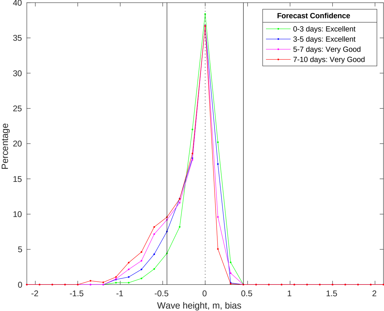
NDBC 52212 vs CMEMS Waves Bias Histogram: 18-Jun-2025
