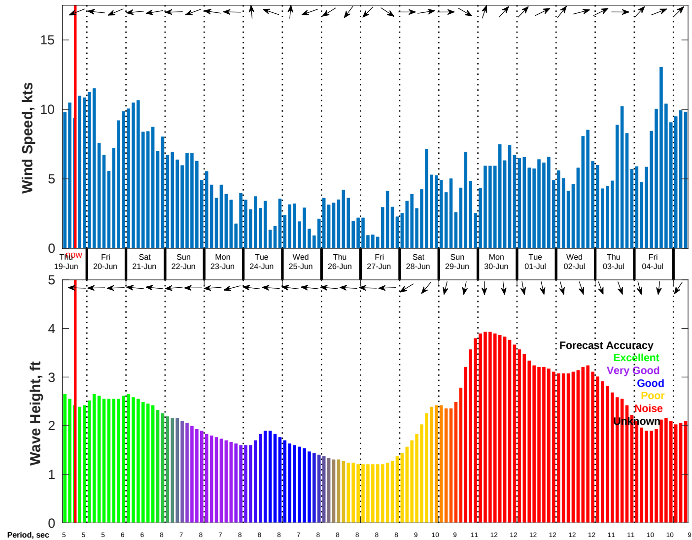
Wind & Wave Forecast for NDBC 52212 from 18-Jun-2025 09:00:00 to 04-Jul-2025 09:00:00
