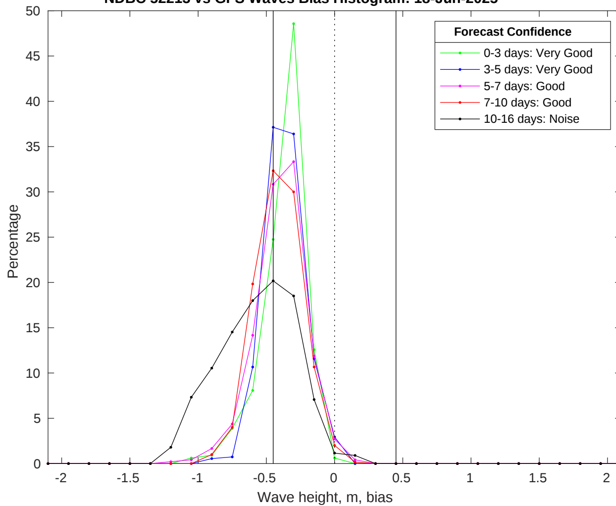
NDBC 52213 vs GFS Waves Bias Histogram: 18-Jun-2025
