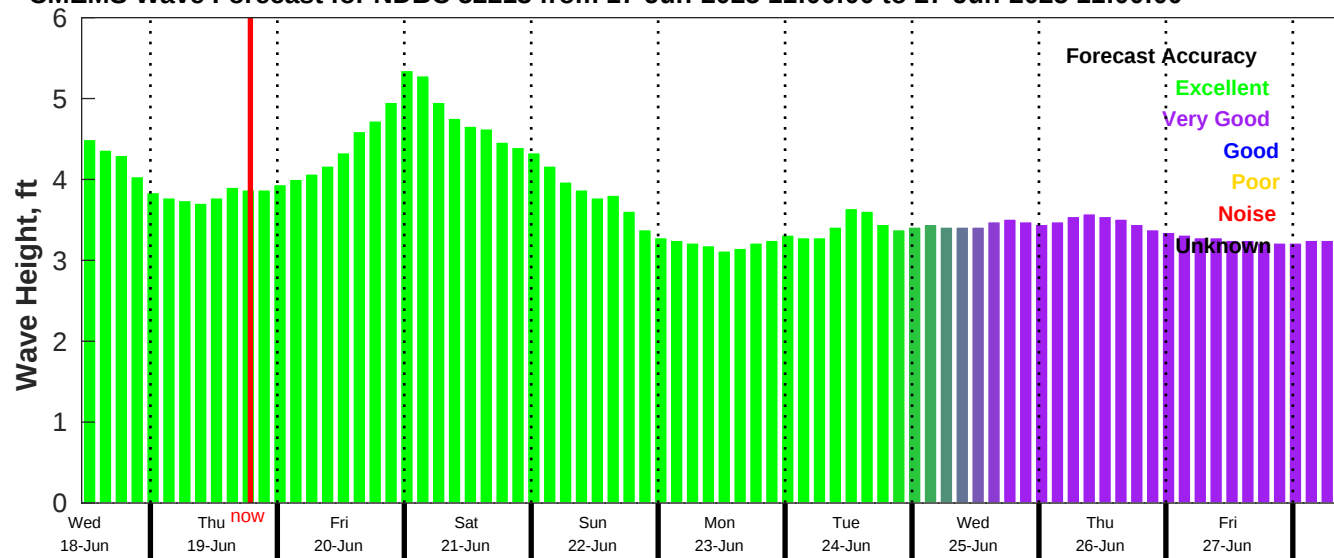
CMEMS Wave Forecast for NDBC 52213 from 17-Jun-2025 11:00:00 to 27-Jun-2025 11:00:00
