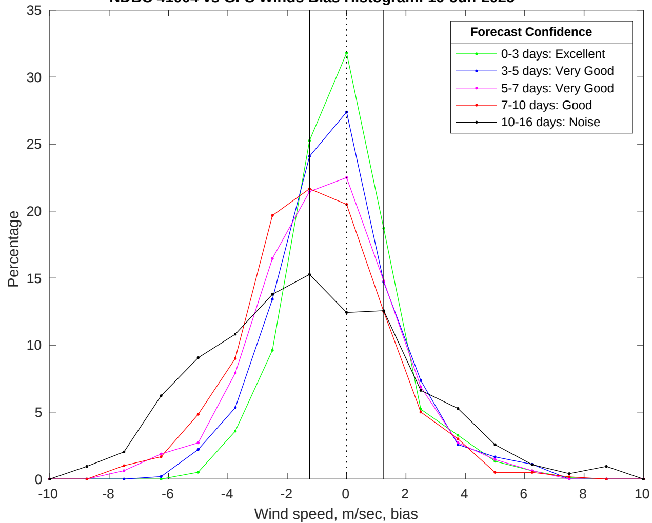
NDBC 41004 vs GFS Winds Bias Histogram: 19-Jun-2025
