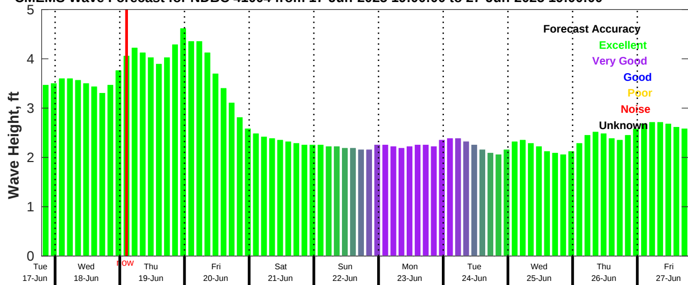
CMEMS Wave Forecast for NDBC 41004 from 17-Jun-2025 19:00:00 to 27-Jun-2025 19:00:00
