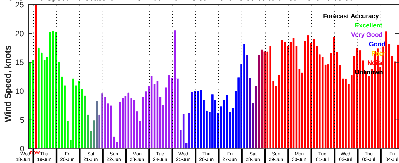
GFS Wind Speed Forecast for NDBC 41004 from 18-Jun-2025 19:00:00 to 04-Jul-2025 19:00:00
