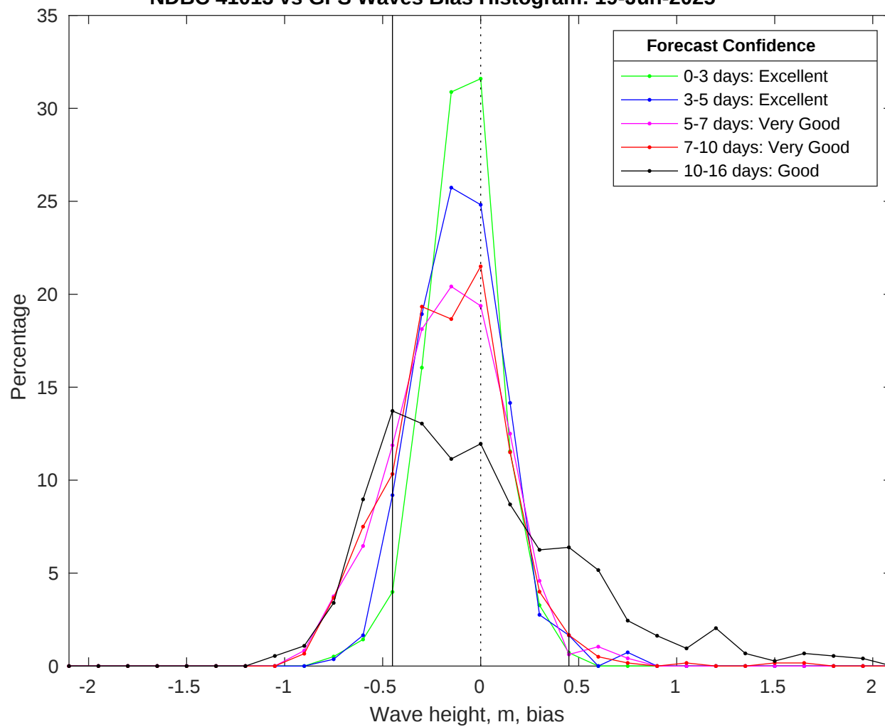
NDBC 41013 vs GFS Waves Bias Histogram: 19-Jun-2025
