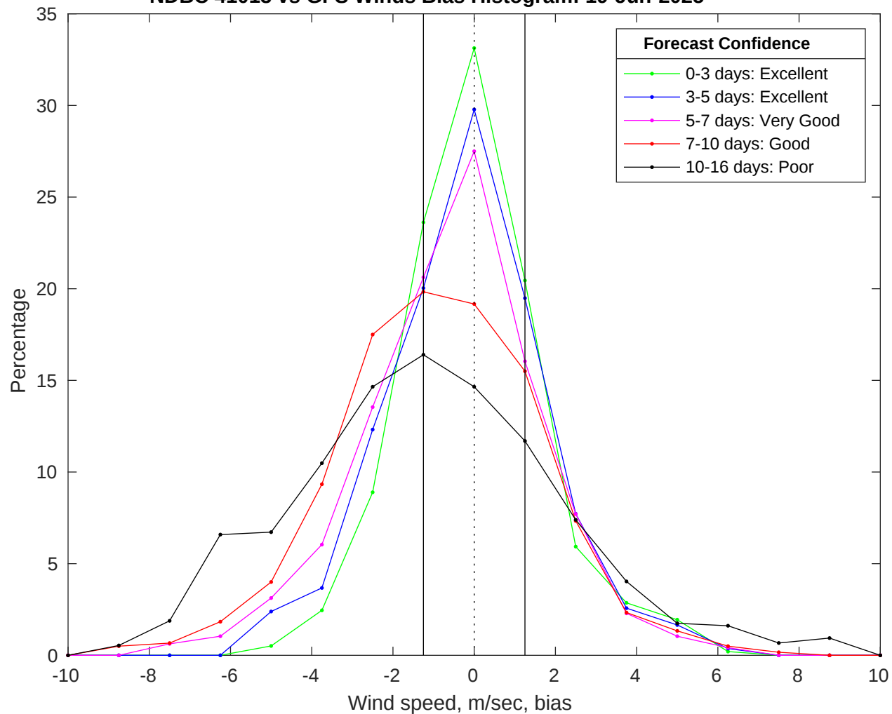
NDBC 41013 vs GFS Winds Bias Histogram: 19-Jun-2025
