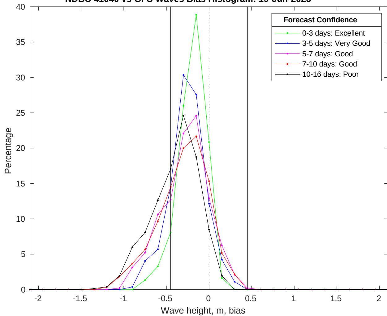
NDBC 41040 vs GFS Waves Bias Histogram: 19-Jun-2025
