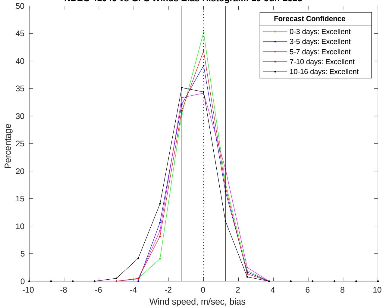
NDBC 41040 vs GFS Winds Bias Histogram: 19-Jun-2025
