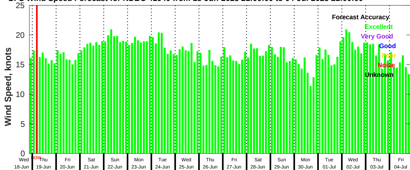
GFS Wind Speed Forecast for NDBC 41040 from 18-Jun-2025 21:00:00 to 04-Jul-2025 21:00:00
