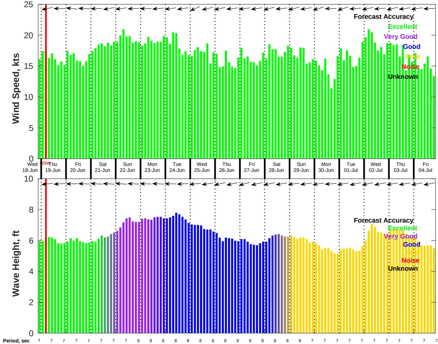
Wind & Wave Forecast for NDBC 41040 from 18-Jun-2025 21:00:00 to 04-Jul-2025 21:00:00
