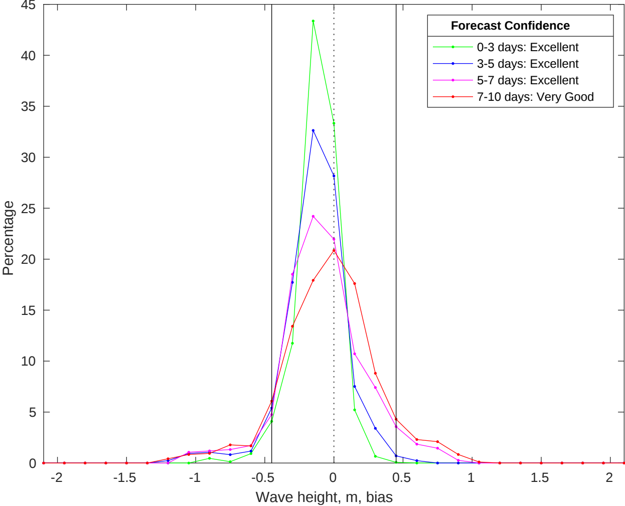
NDBC 42019 vs CMEMS Waves Bias Histogram: 19-Jun-2025
