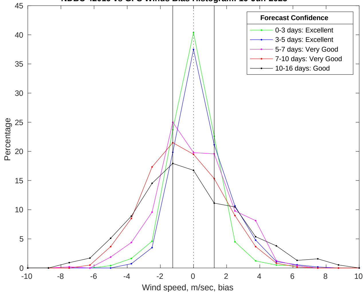
NDBC 42019 vs GFS Winds Bias Histogram: 19-Jun-2025
