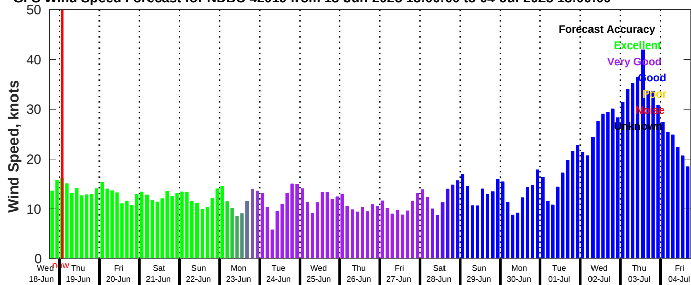
GFS Wind Speed Forecast for NDBC 42019 from 18-Jun-2025 18:00:00 to 04-Jul-2025 18:00:00
