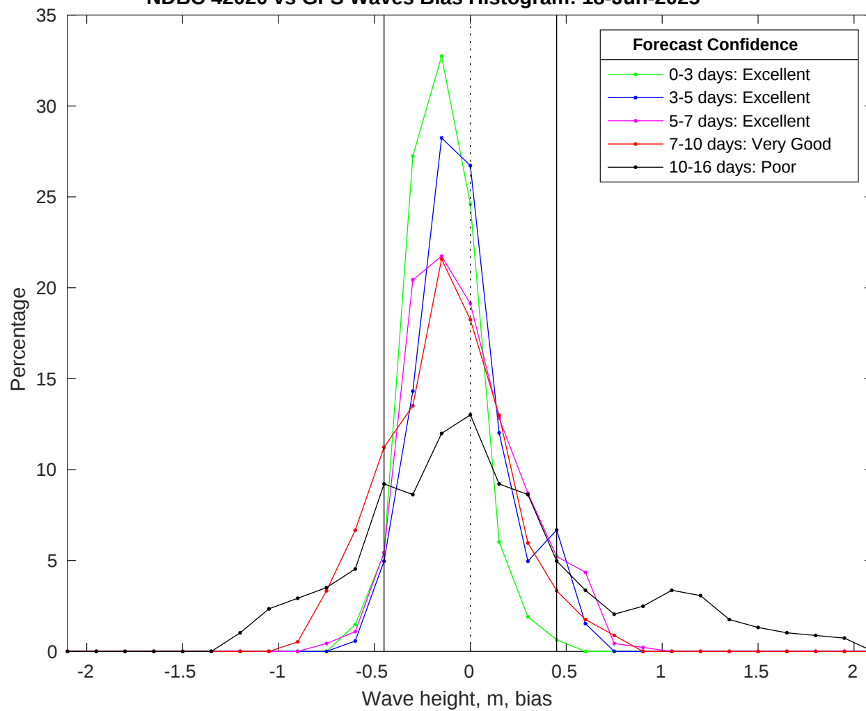
NDBC 42020 vs GFS Waves Bias Histogram: 18-Jun-2025
