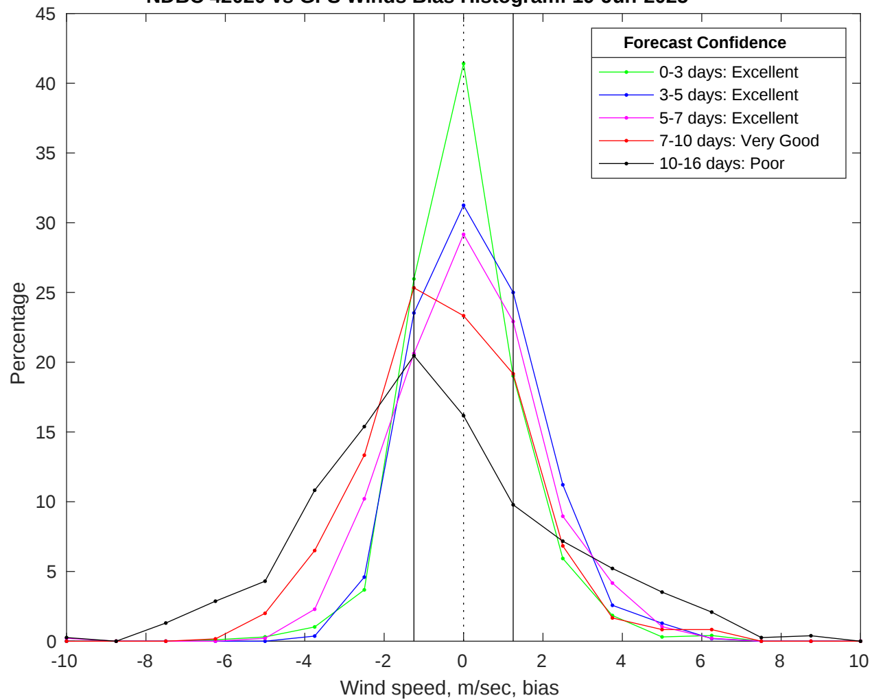
NDBC 42020 vs GFS Winds Bias Histogram: 19-Jun-2025
