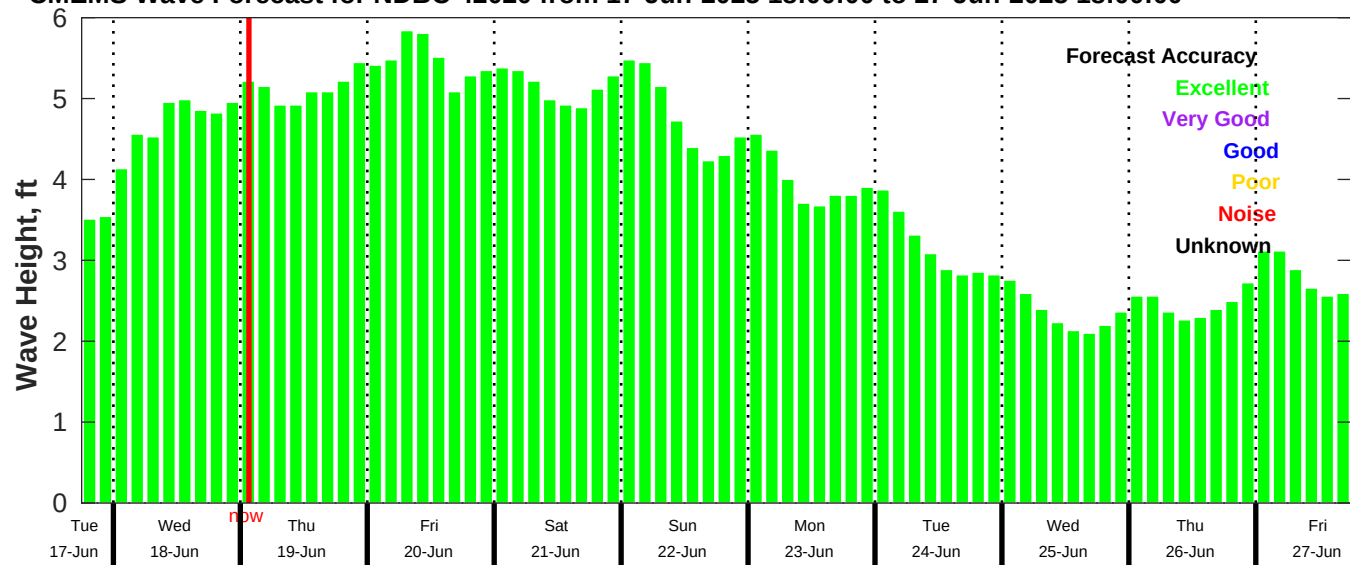
CMEMS Wave Forecast for NDBC 42020 from 17-Jun-2025 18:00:00 to 27-Jun-2025 18:00:00
